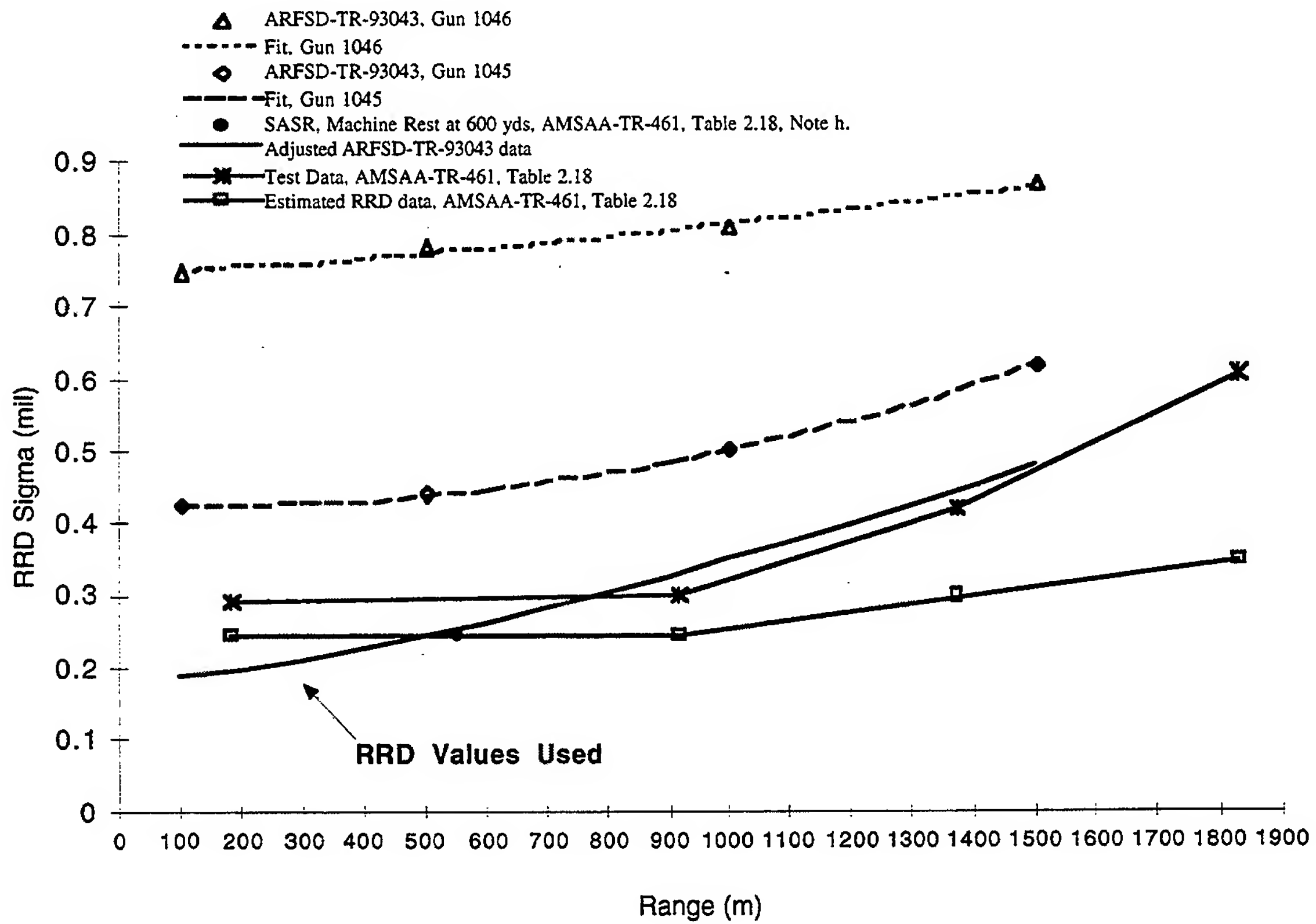
Figure A-2. RRD Data, 50 CAL MK211.
